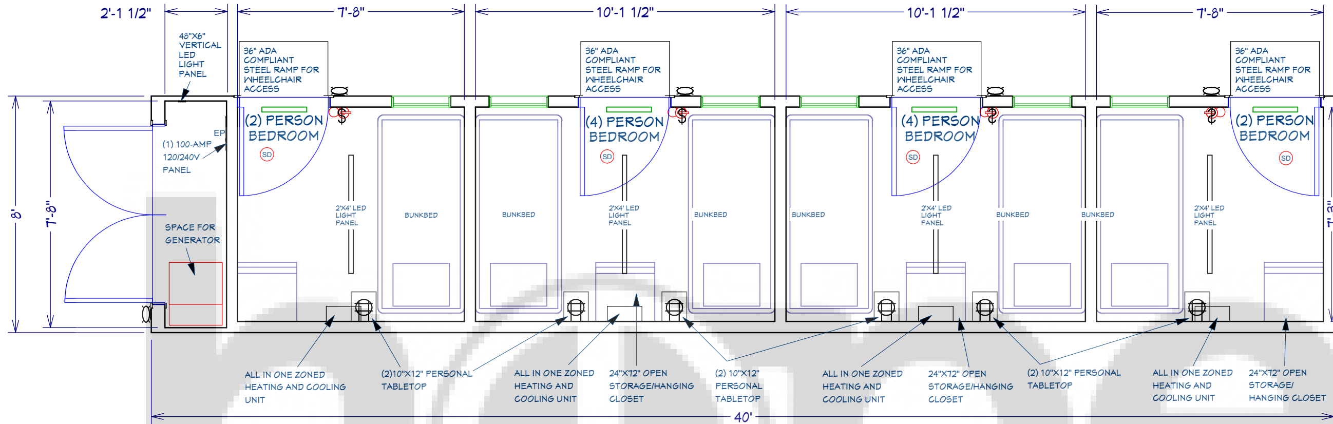
FLOOR PLAN NTS
