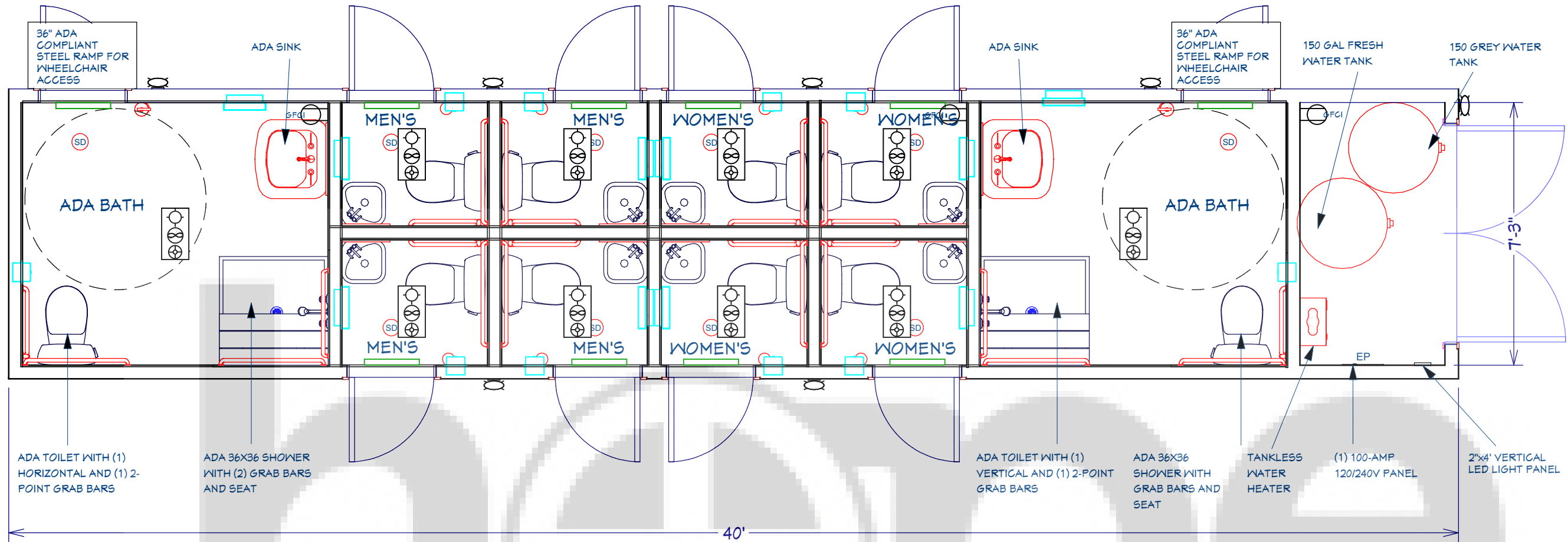
FLOOR PLAN NTS
